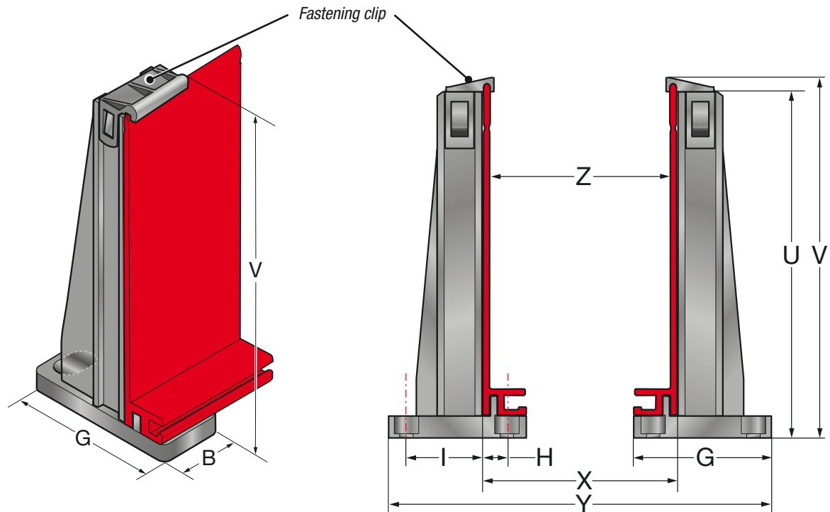
Guide channel side section
